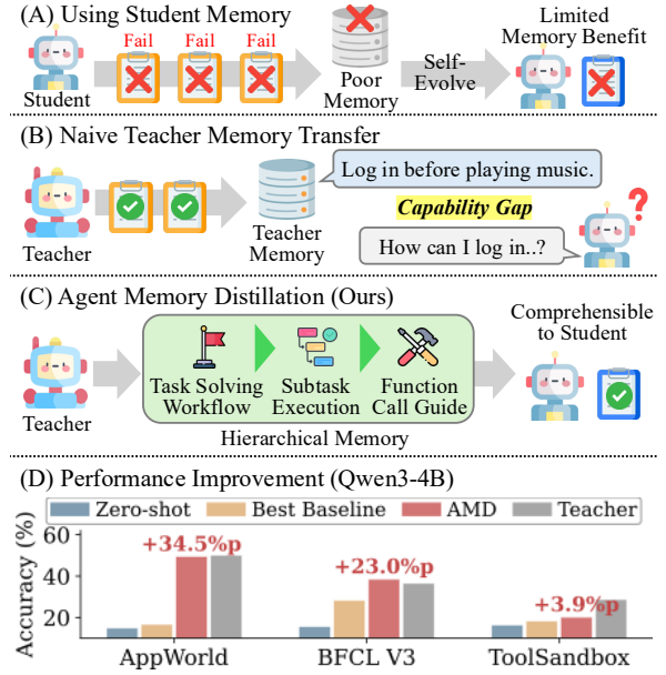
Figure 1: Motivation, Concept, and Results of AMD. (A) Student-generated memory is limited by low task success rates. (B) Naive teacher memory transfer yields marginal gains due to the capability gap. (C) AMD transfers hierarchical memories spanning task, subtask, and function levels, making teacher knowledge accessible to small students. (D) AMD achieves significant accuracy gains across three benchmarks.
