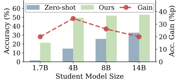
Figure 4: Effect of student model size on AMD performance. Accuracy increases with model size, while accuracy gain peaks at 4B.
