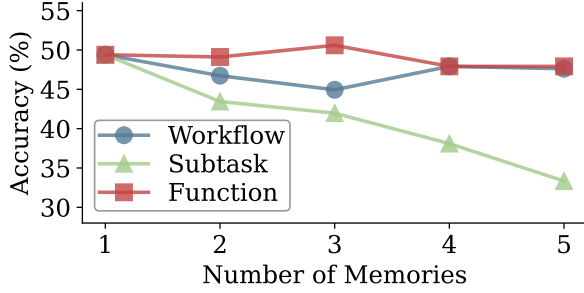
Figure 5: Effect of retrieval count k on AMD performance. Accuracy at k=1 is near-optimal for all memory types, and increasing k generally degrades performance.
