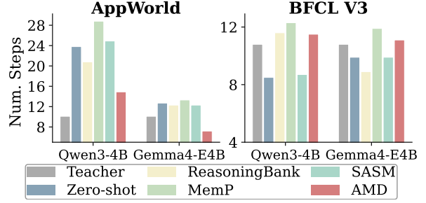
Figure 3: Interaction steps on two benchmarks. AMD brings the student’s turn count closer to the teacher’s, particularly where the zero-shot gap is large.
