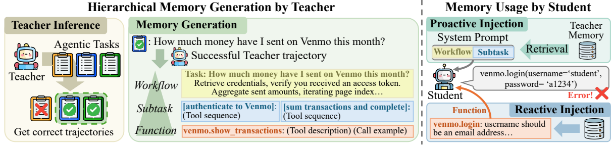
Figure 2: Hierarchical Memory Generation and Injection in AMD. (Left) The teacher agent generates three types of memory from successful trajectories. (Right) At inference time, Workflow and Subtask memories are proactively injected into the system prompt, while Function memory is reactively retrieved upon tool-calling errors.
